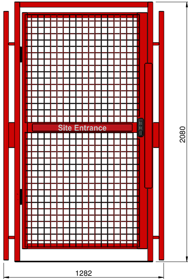
VIEW ON FRONT OF GATE
